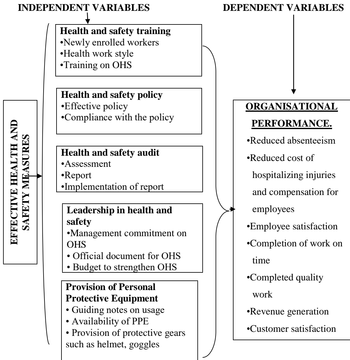
Figure 2.1: Conceptual Framework
